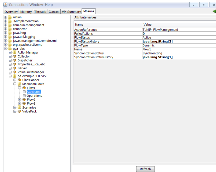
Figure 18 - Java JMX Console: UCA for EBC Value Pack – Mediation Flows - Attributes
